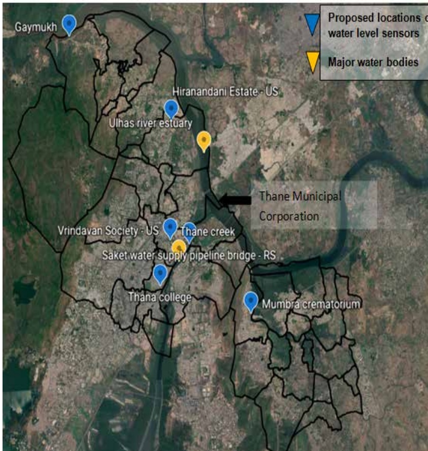
Figure 4. Location of real-time water level sensors
